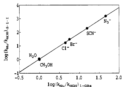
Figure 8. Comparison of nucleophilic selectivities toward d -1-I and 1-OBs in 25 vol % acetonitrile in water ( \mu = 0.75 M, maintained with NaClO 4 ) at 70 and 35 °C, respectively.
